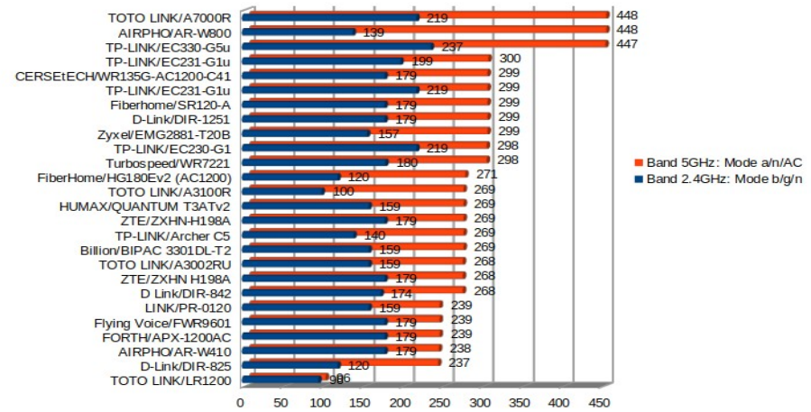
WiFi Capacity vs Concurrent TCP Throughput (Mbps)
