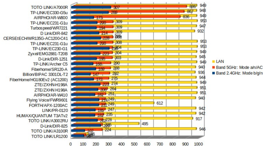
UDP Throughput Rate (Mbps)
