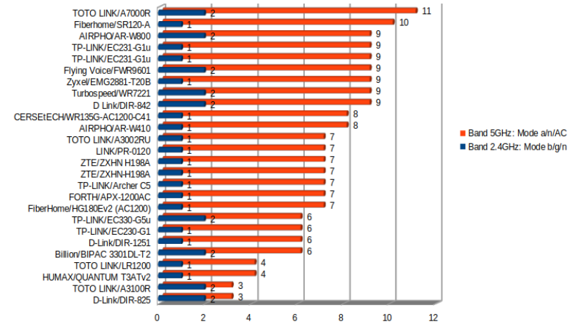
WiFi Capacity vs Concurrent TCP Throughput (Mbps)
