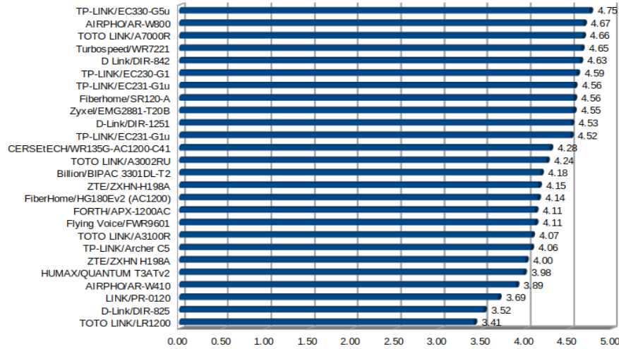
UDP Throughput Rate (Mbps)
